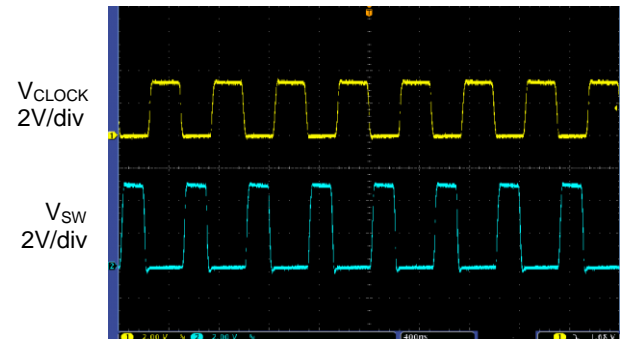
Time 400ns/div
